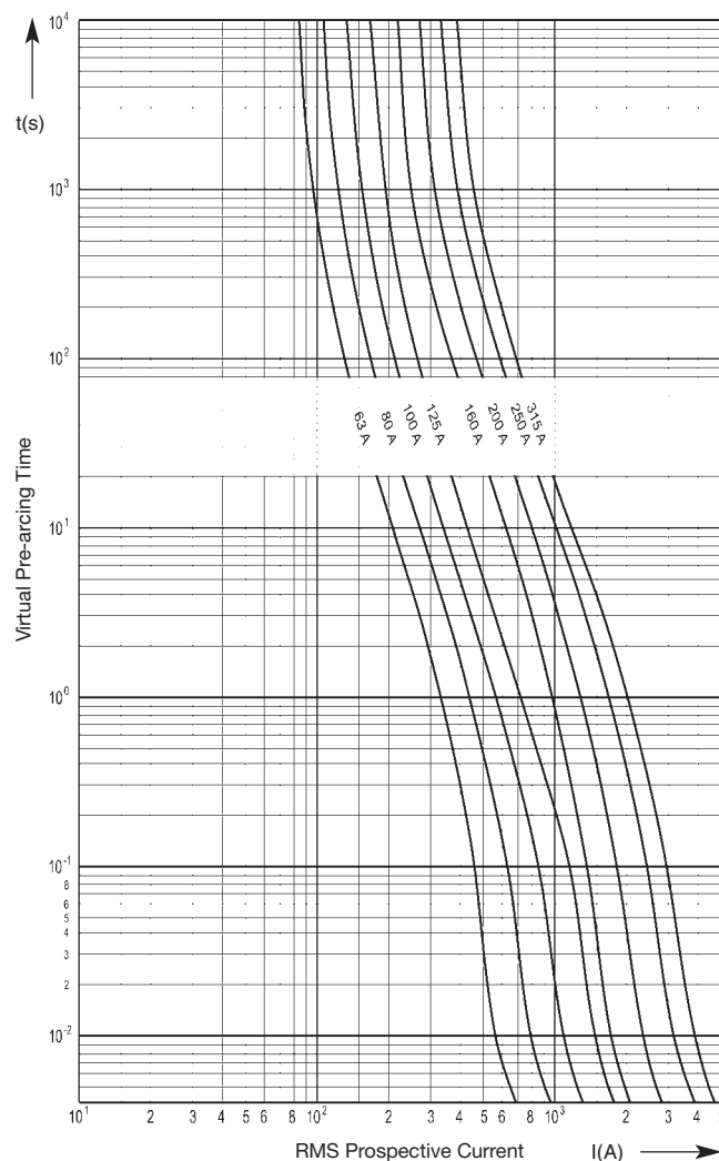
Time-Current Characteristics
