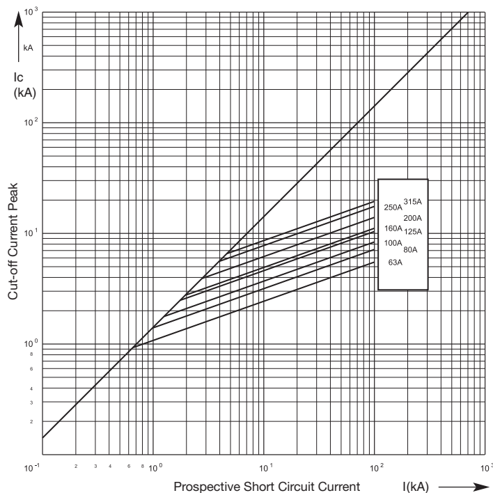
Cut-Off Characteristics
