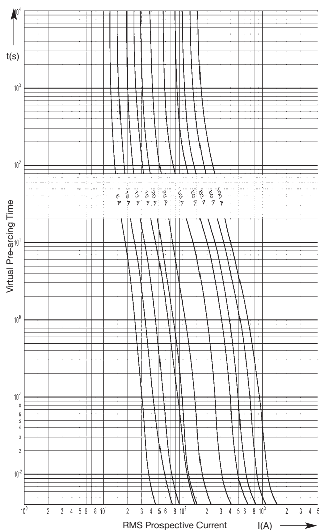
Time-Current Characteristics
