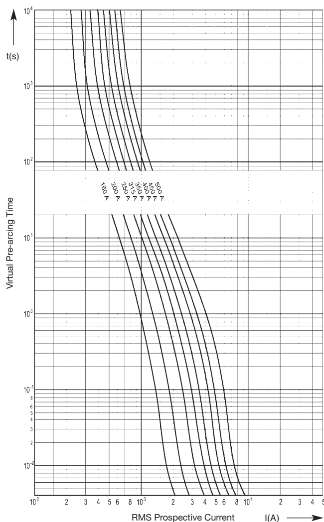
Time-Current Characteristics
