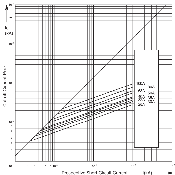
Cut-Off Characteristics
