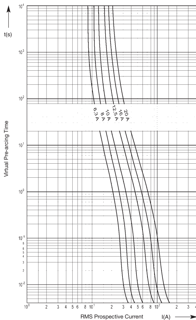
Time-Current Characteristics
