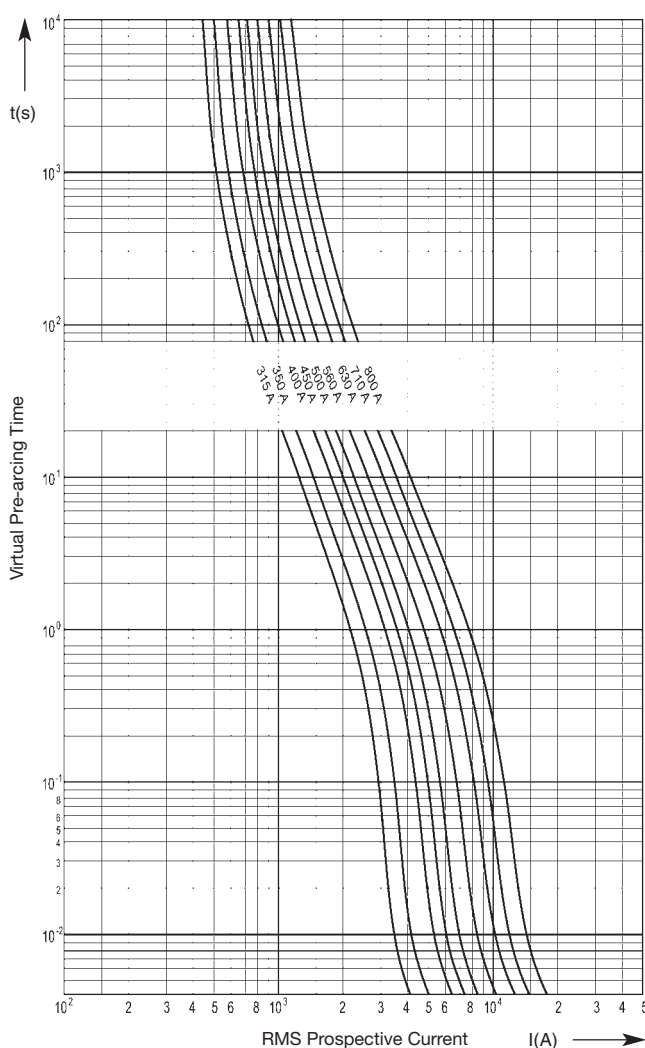
Time-Current Characteristics
